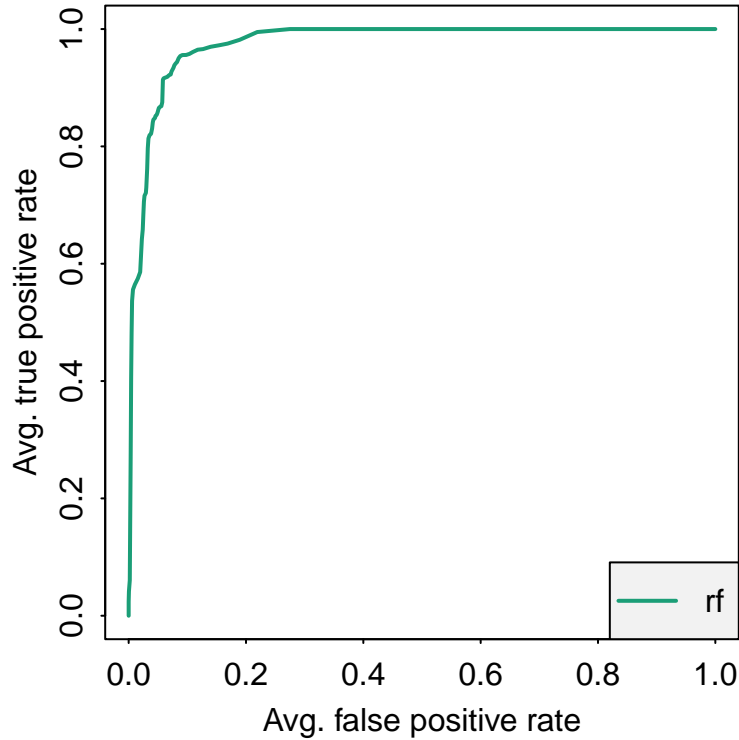
Figure 2. ROC plot for all 22 validation runs, averaged along cutoffs, for each modeling algorithm.
