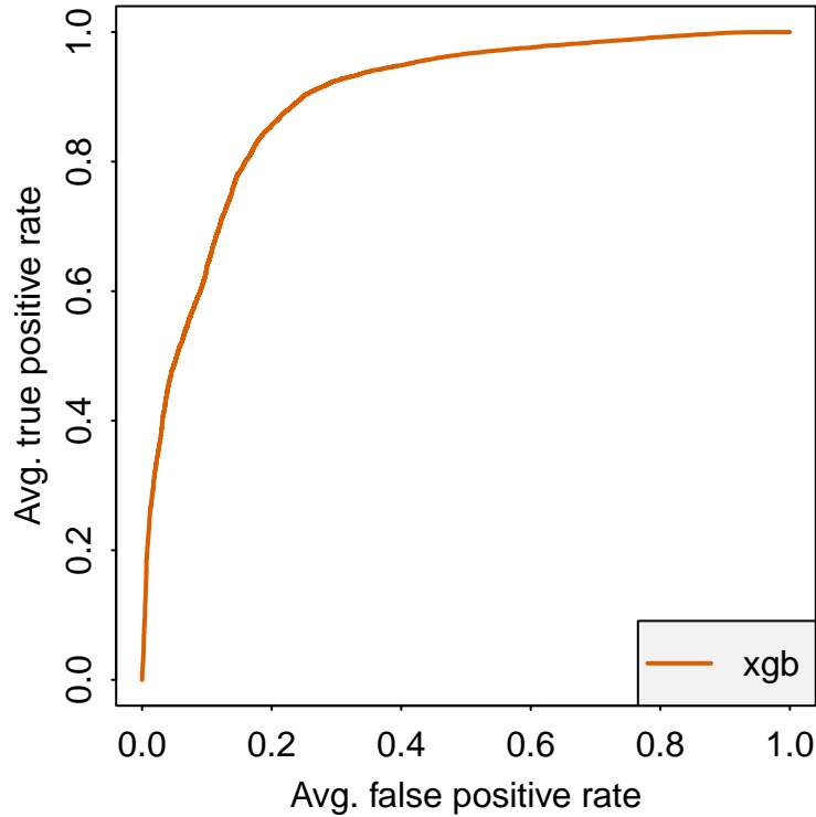
Figure 2. ROC plot for all 30 validation runs, averaged along cutoffs, for each modeling algorithm.
