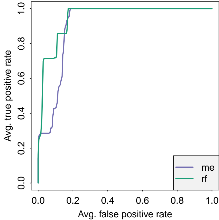
Figure 2. ROC plot for all 7 validation runs, averaged along cutoffs, for each modeling algorithm.
