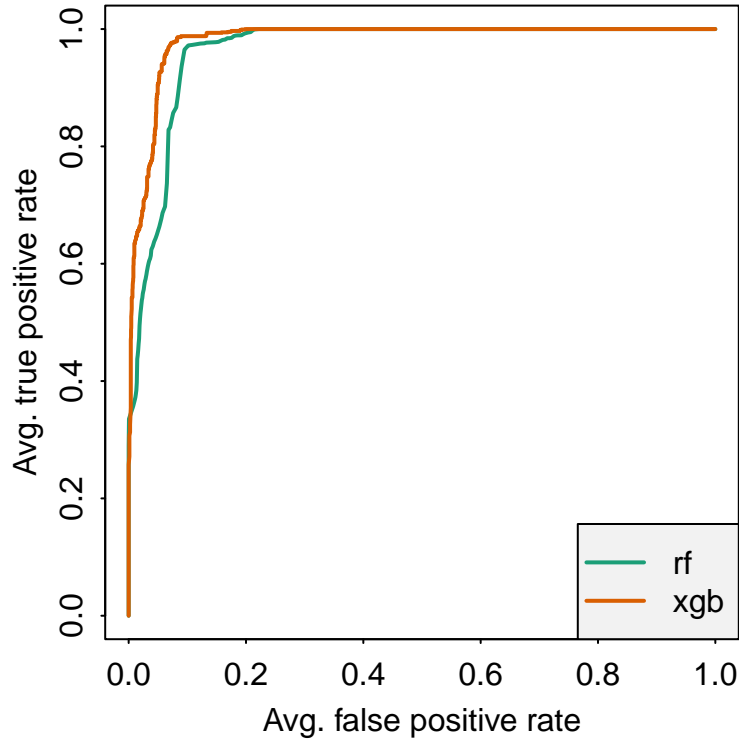
Figure 2. ROC plot for all 6 validation runs, averaged along cutoffs, for each modeling algorithm.
