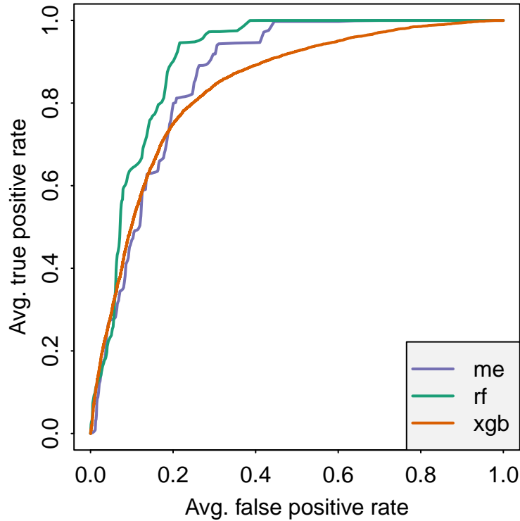
Figure 2. ROC plot for all 37 validation runs, averaged along cutoffs, for each modeling algorithm.
