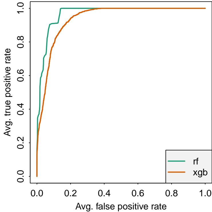
Figure 2. ROC plot for all 11 validation runs, averaged along cutoffs, for each modeling algorithm.
