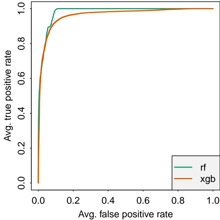
Figure 2. ROC plot for all 48 validation runs, averaged along cutoffs, for each modeling algorithm.
