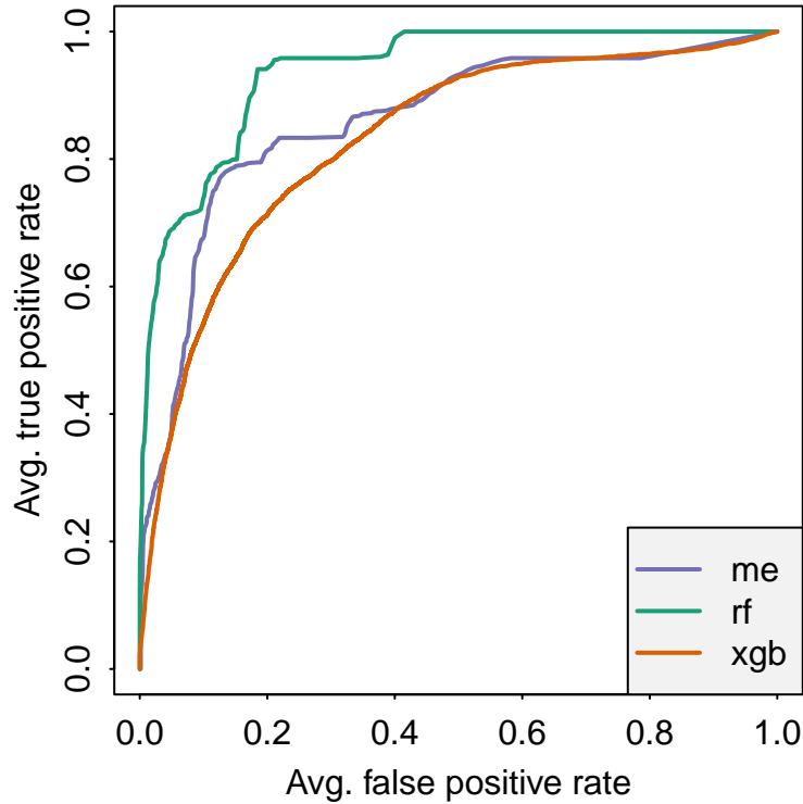
Figure 2. ROC plot for all 24 validation runs, averaged along cutoffs, for each modeling algorithm.
